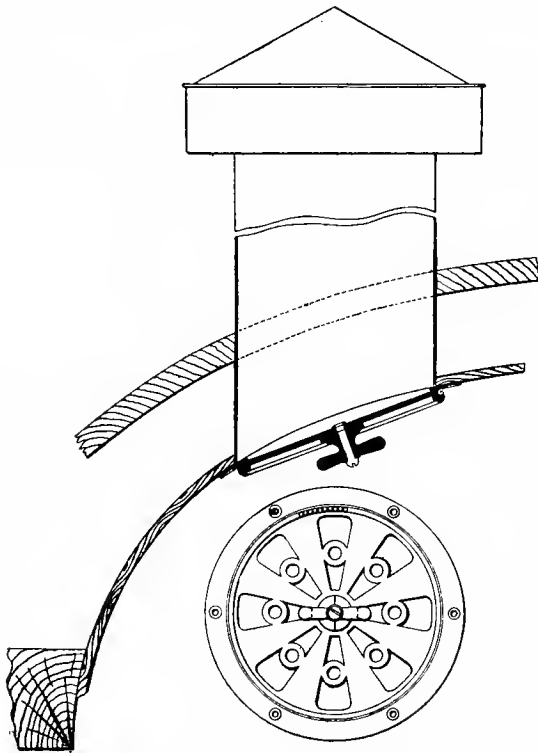
Fig. 4325-5. VENTILATOR FOR SALOONS.
